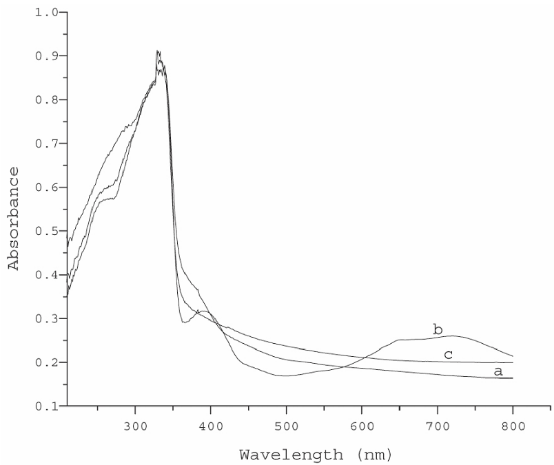
Figure S2. UV-Vis absorption spectra of 1 (a), 2 (b), and 3 (c).
