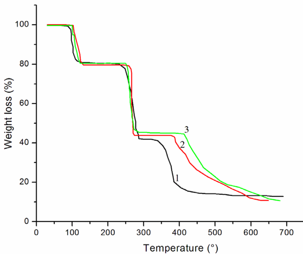
Figure S1. TGA curves of 1 (a), 2 (b) and 3 (c).
